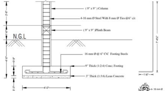
(F) FOOTING SECTION (TYPICAL)
